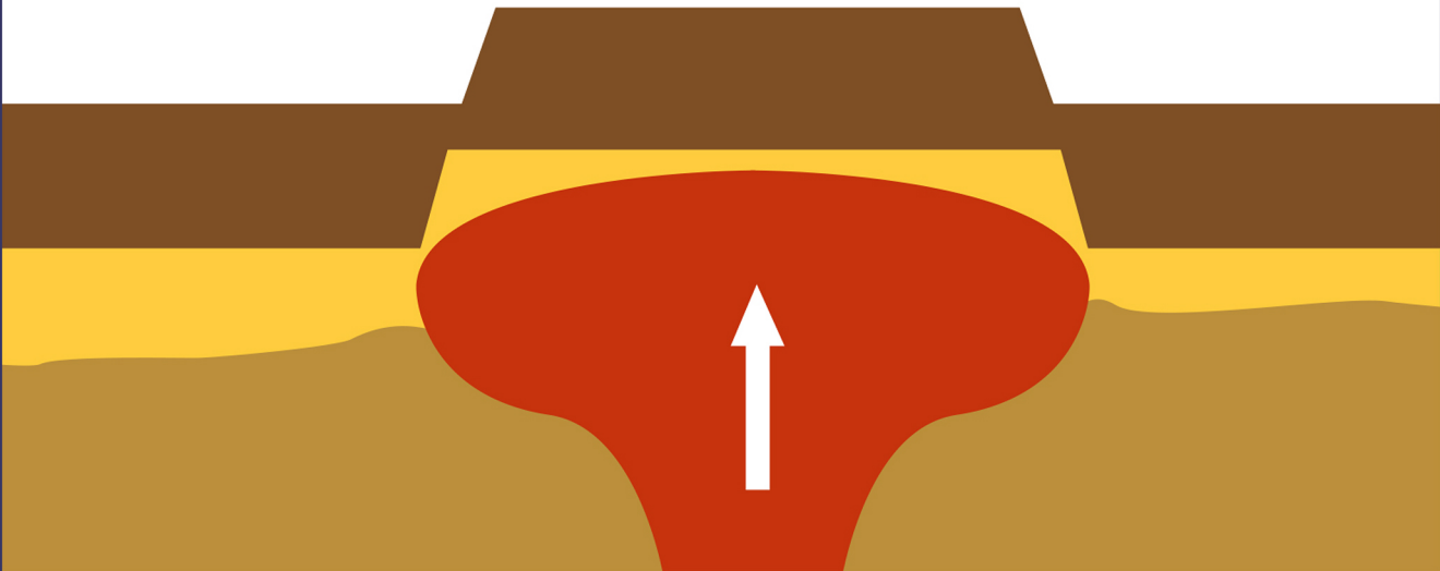
erosional mountain
