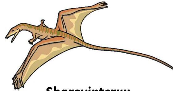
Sharovipteryx
